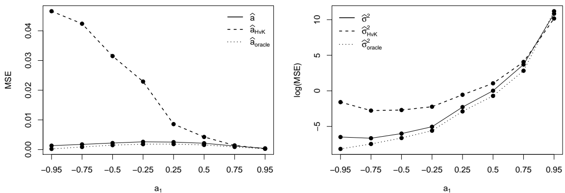
Figure 5: MSE values for the estimators \hat{a} , \hat{a}_{\text{HvK}} , \hat{a}_{\text{oracle}} and \hat{\sigma}^2 , \hat{\sigma}_{\text{HvK}}^2 , \hat{\sigma}_{\text{oracle}}^2 in the simulation scenarios with a pronounced trend ( s_\beta = 10 ).
